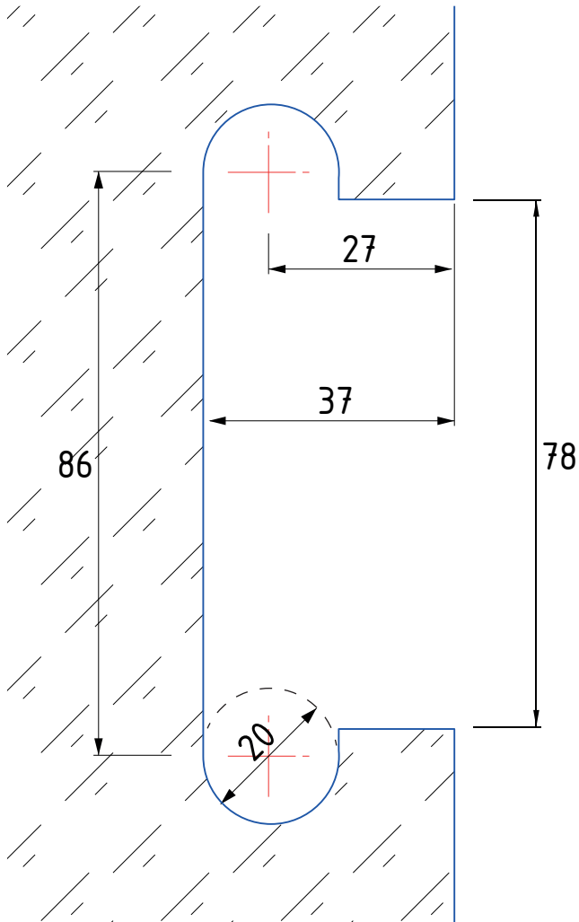
SJ1L Cutout Detail (Differs from Glass to Glass cuout)
