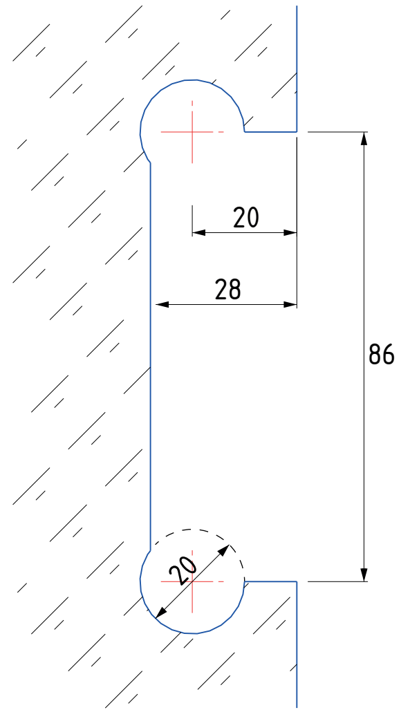
SJ2 Cutout Detail (Differs from Glass to Wall cuout)
